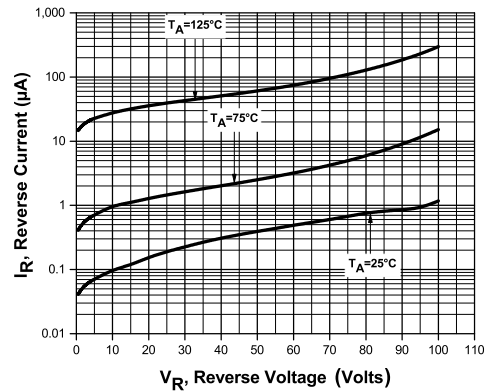
Leakage Current for CMSH2-100M
